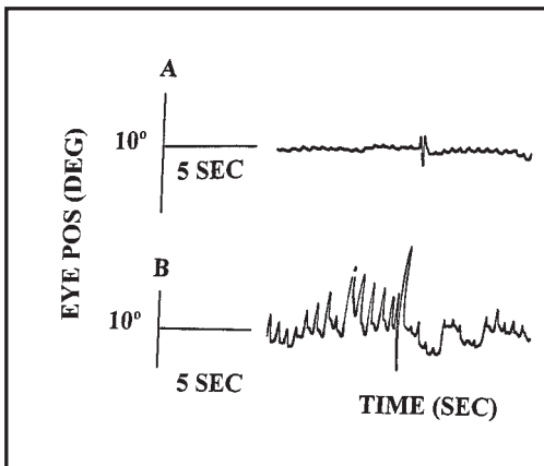
Figure 2. Horizontal eye position as a function of time. Follow-up test session, one week later. (A) with SCL. (B) with SCL and anesthetic. Upward deflection indicates leftward nystagmoid movement, and downward deflection indicates rightward nystagmoid movement.
