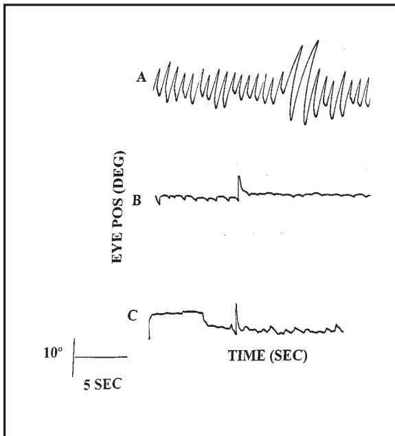
Figure 1. Figure 1: Horizontal eye position as a function of time. Initial test session. (A) with spectacles. (B) with SCL. (C) with SCL and anesthetic. Upward deflection indicates leftward nystagmoid movement, and downward deflection indicates rightward nystagmoid movement.
