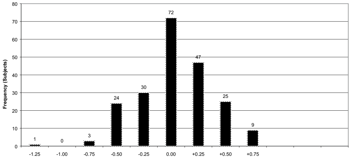
Figure 3. Frequency distribution of MEM PLA results, right eye.
