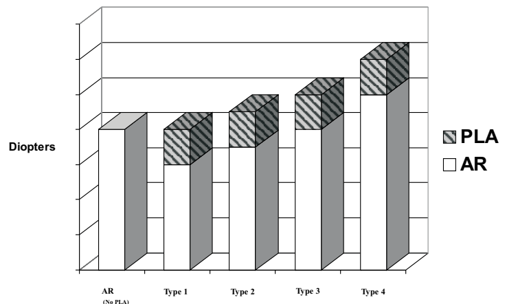
Figure 1. Four types of changes in accommodative response (AR) when a plus lens addition (PLA) is introduced. The extreme left bar is the AR without a PLA.
