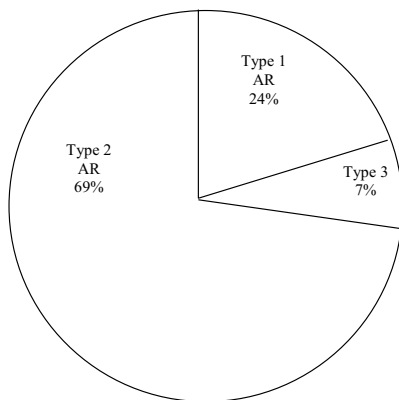
Figure 4. Distribution of AR changes with PLA in place.
