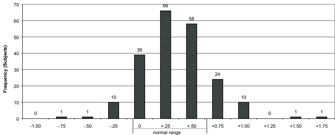
Figure 2. Histogram showing the frequency distribution of MEM values for the right eye of all subjects. (N=211)
